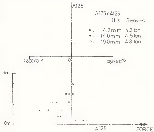
Fig. 6 Strain Distribution
